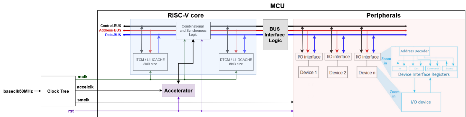
Figure 1 : MCU System General Architecture
