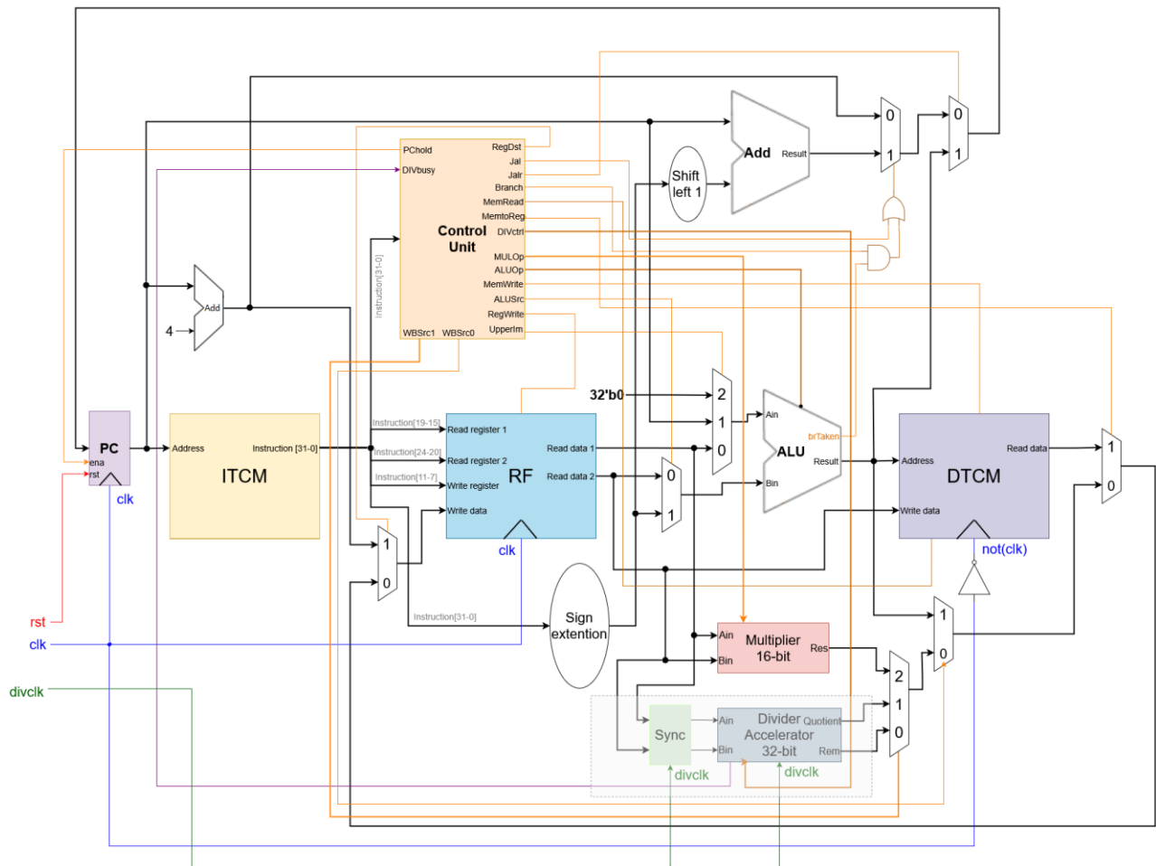
Figure 3: RV32IM single-cycle core connected to a divider accelerator
