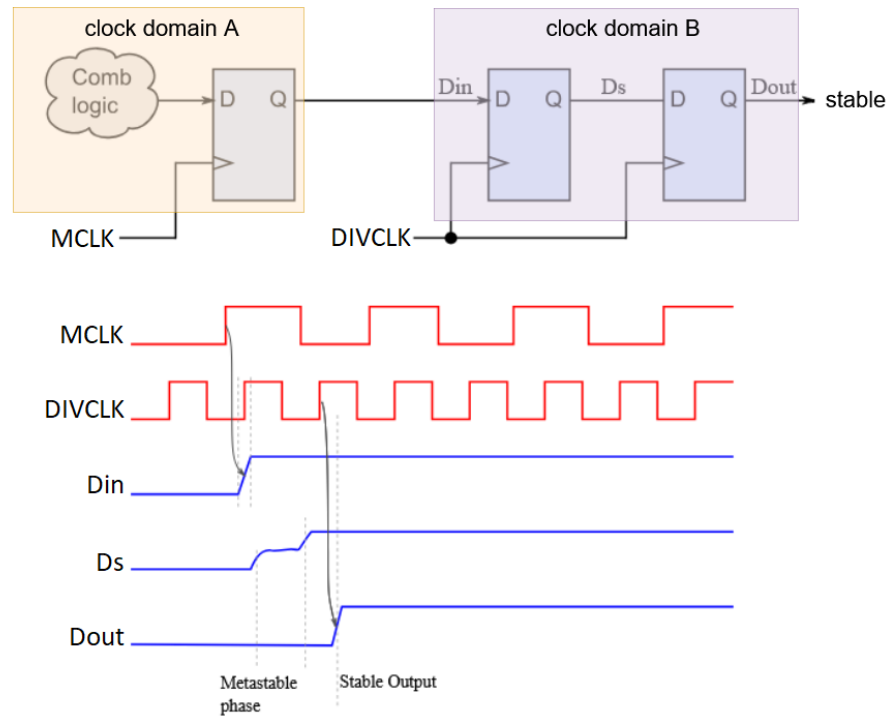
Figure 10: CDC (clock domain crossing) synchronizer
