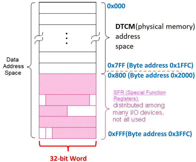
Figure 2: Data Address Space contains Data Memory and I/O Memory Mapped I/O
